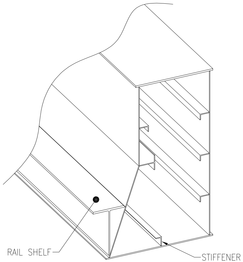
TYPICAL BOOM GIRDER SHAPE
